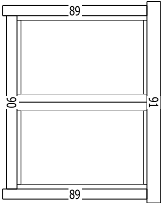
DOUBLE WINDOW 1380X1050
